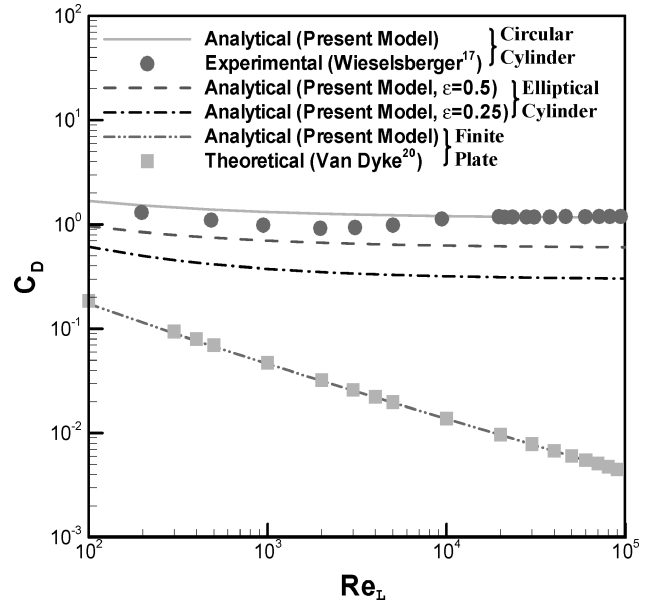
Fig. 4 Variation of total drag coefficient with Reynolds number.
